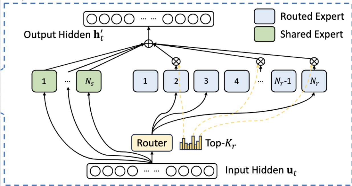
DeepSeekMoE
